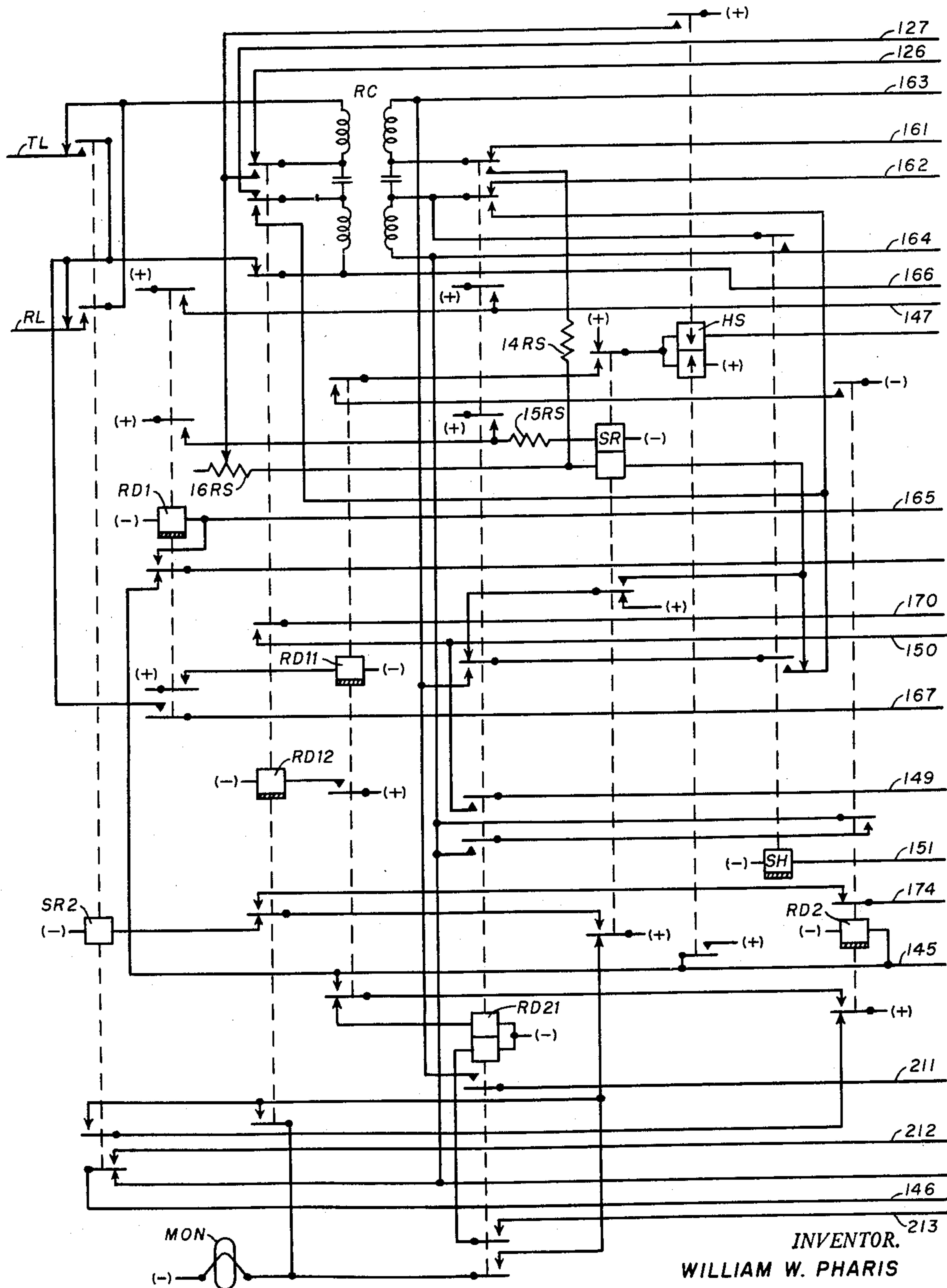
2-WAY F.S. AND TOLL REPEATER TANDEM OFFICE
