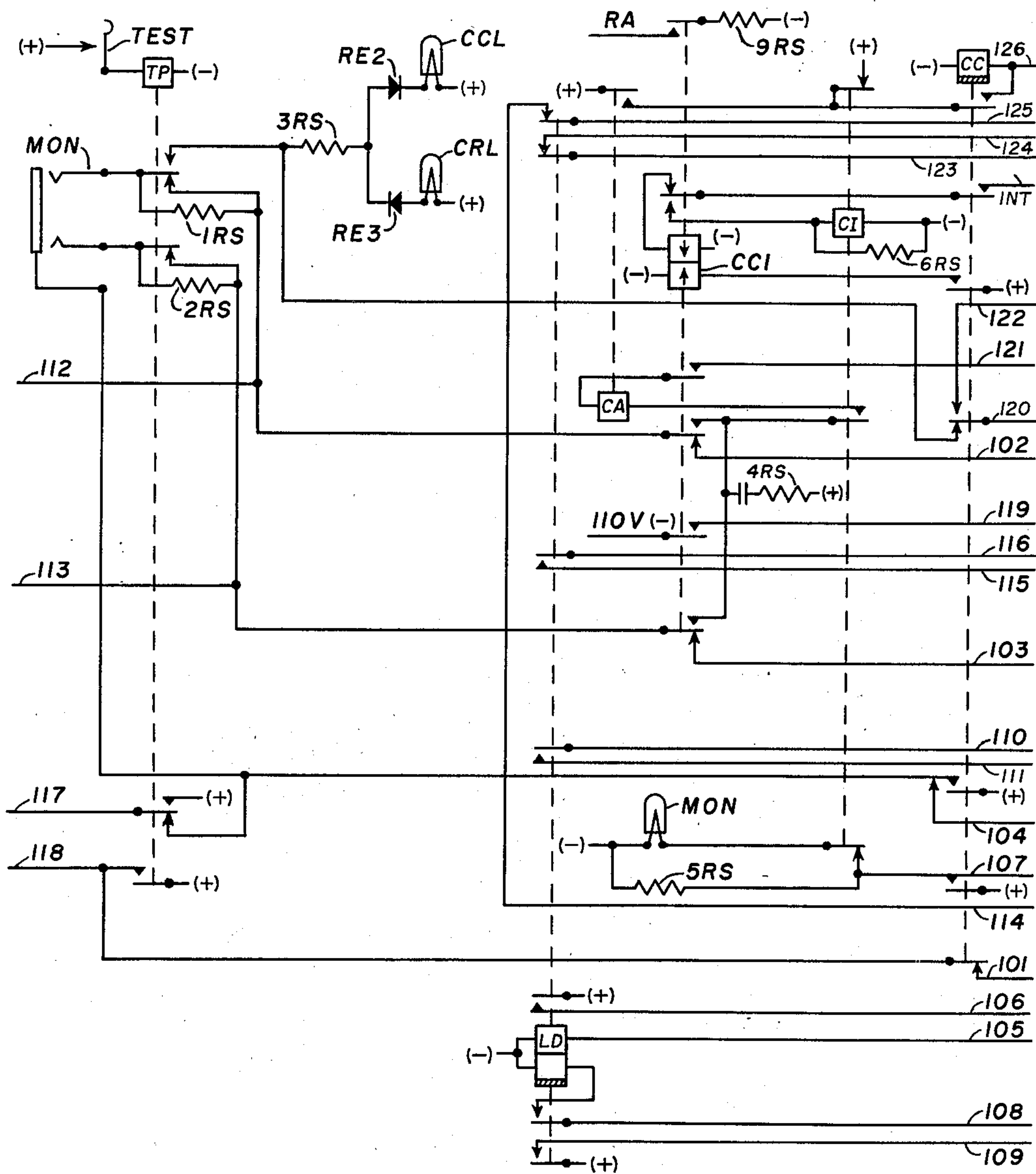
PAY STATION ADAPTER
