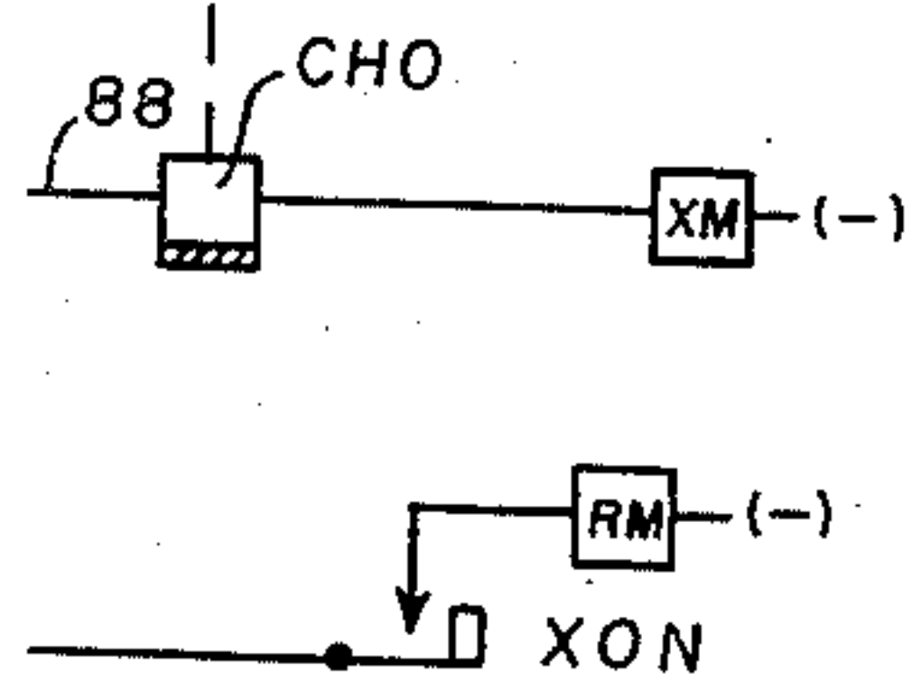
1ST SELECTOR
