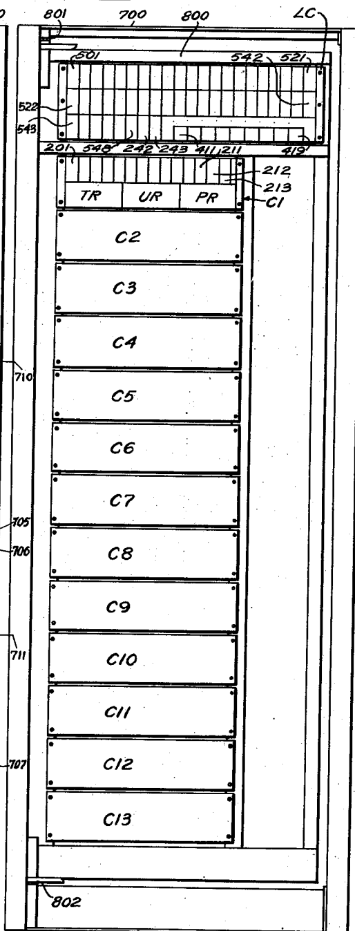
Fig. 8 (Rear)
