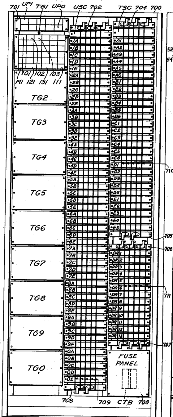
Fig. 7 (Front)
