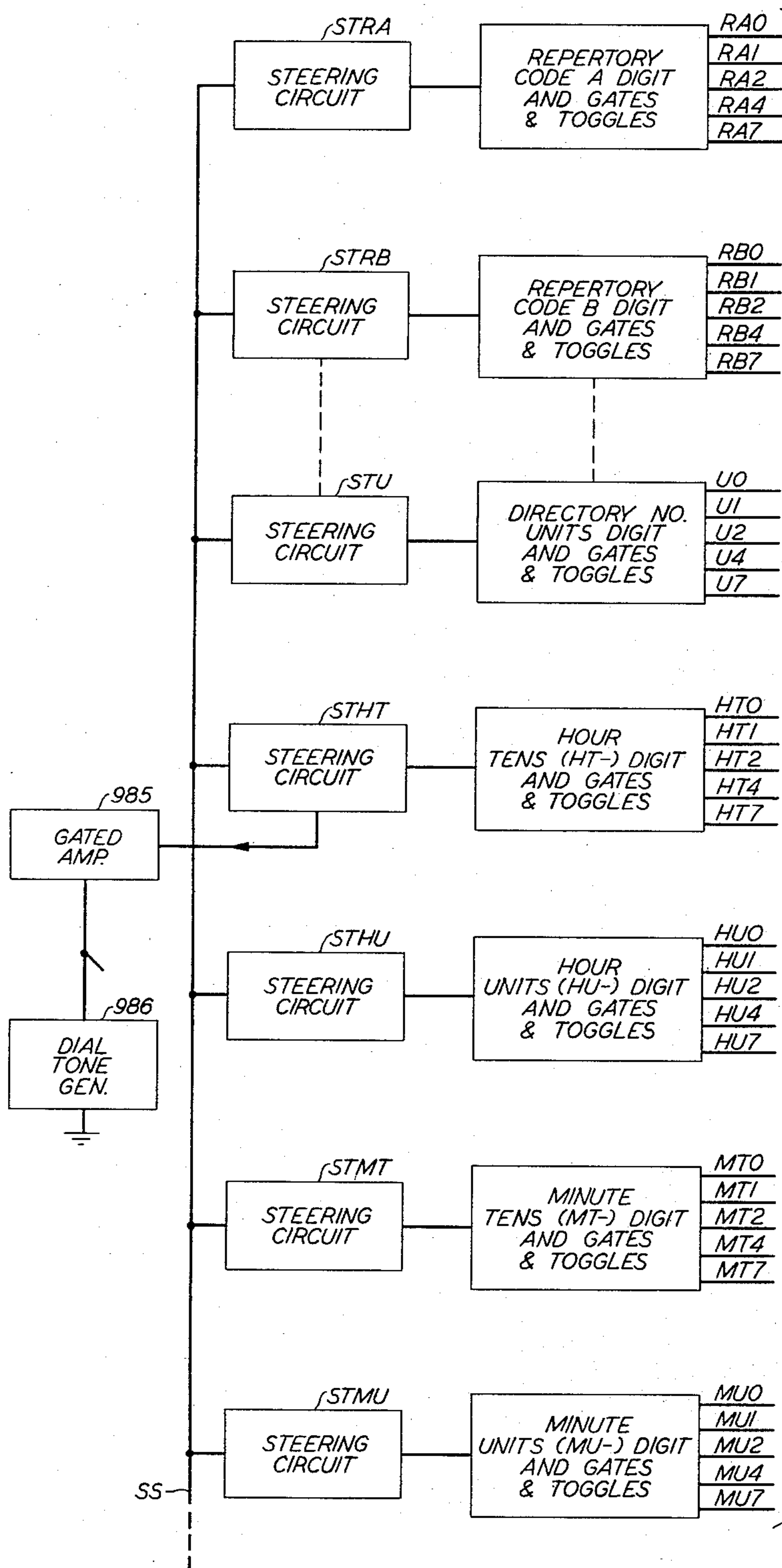
FIG. 3 REPERTORY CHANGE REGISTER TRUNK 22
