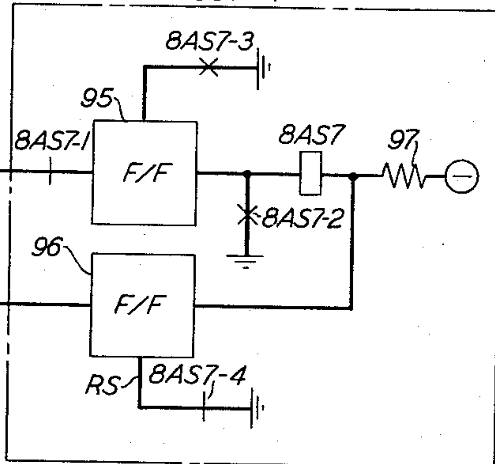
TRANSFER CCT. 7
