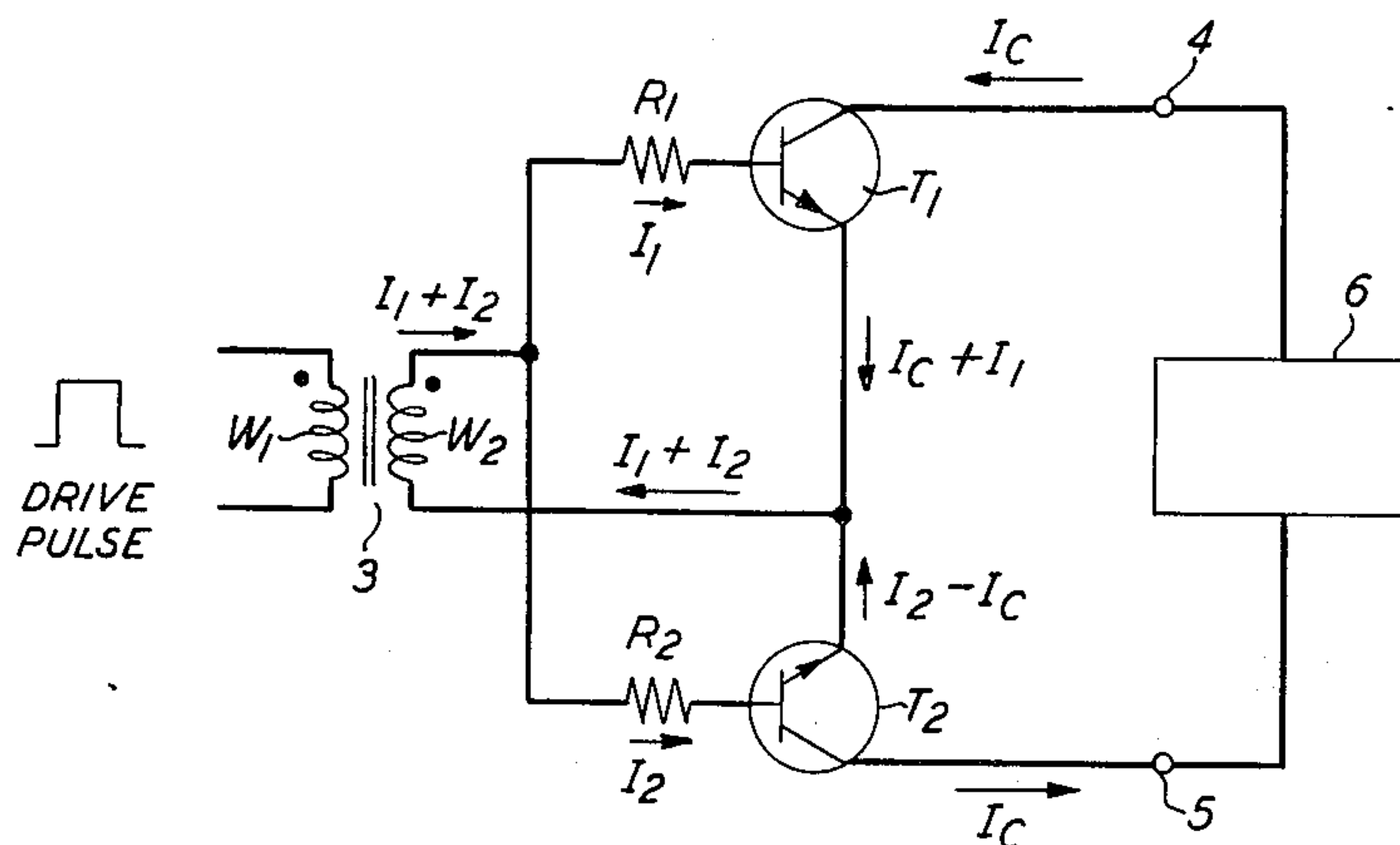
PRIOR ART TWO-TRANSISTOR SWITCH
