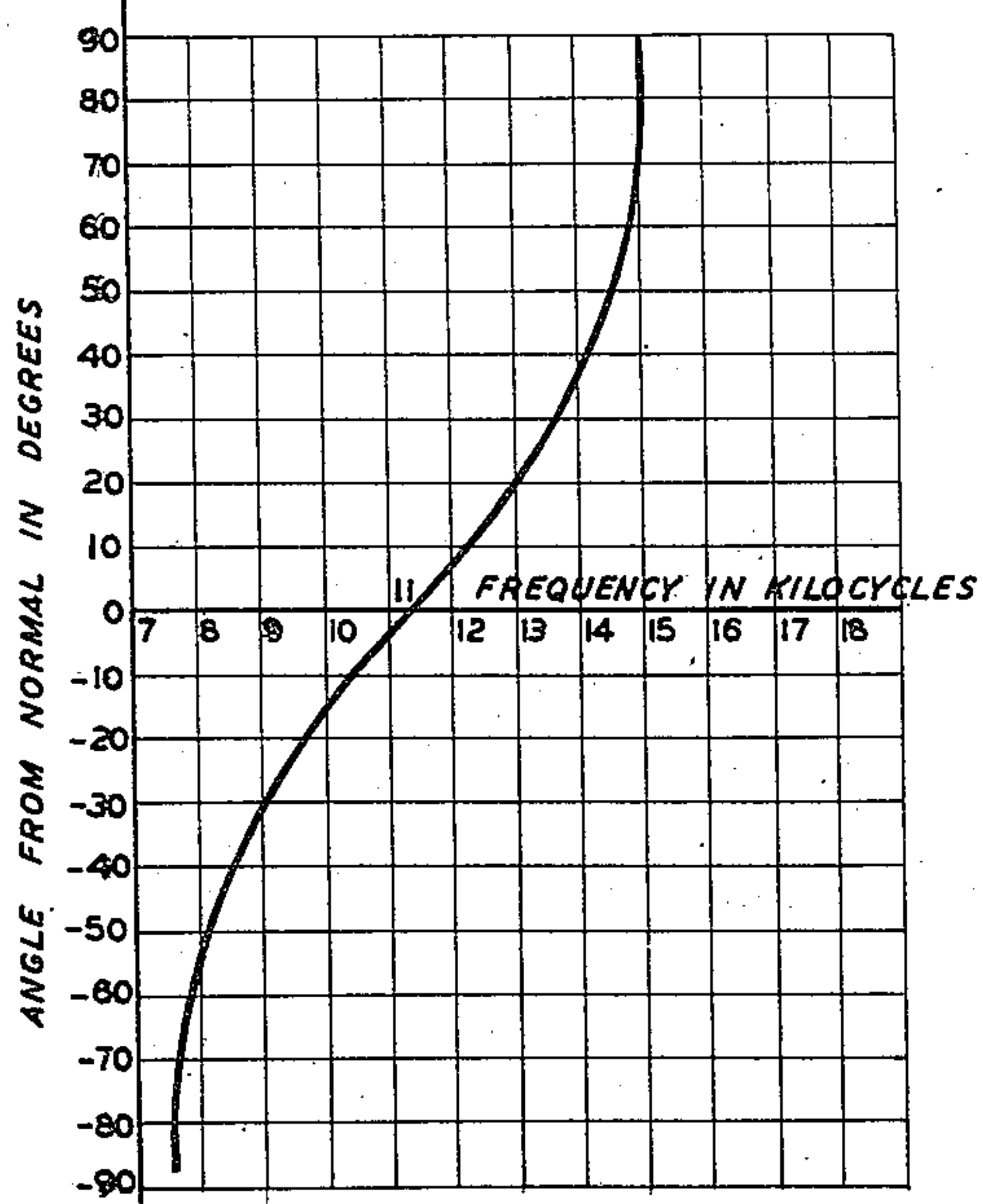
ANGLE FREQUENCY CURVE FOR SUPERSONIC PRISM
