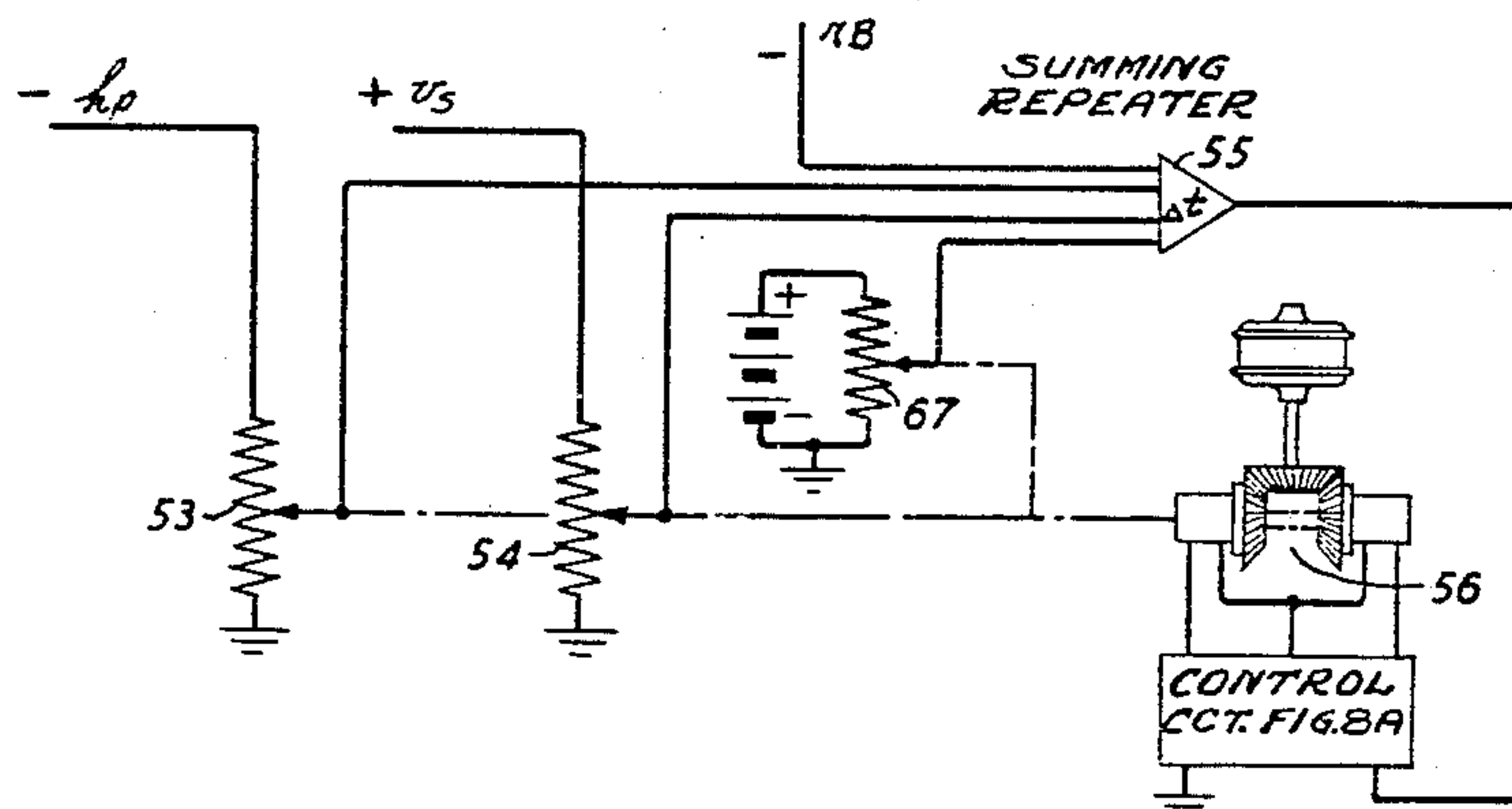
FIG. 10 BALLISTIC CONVERTER
