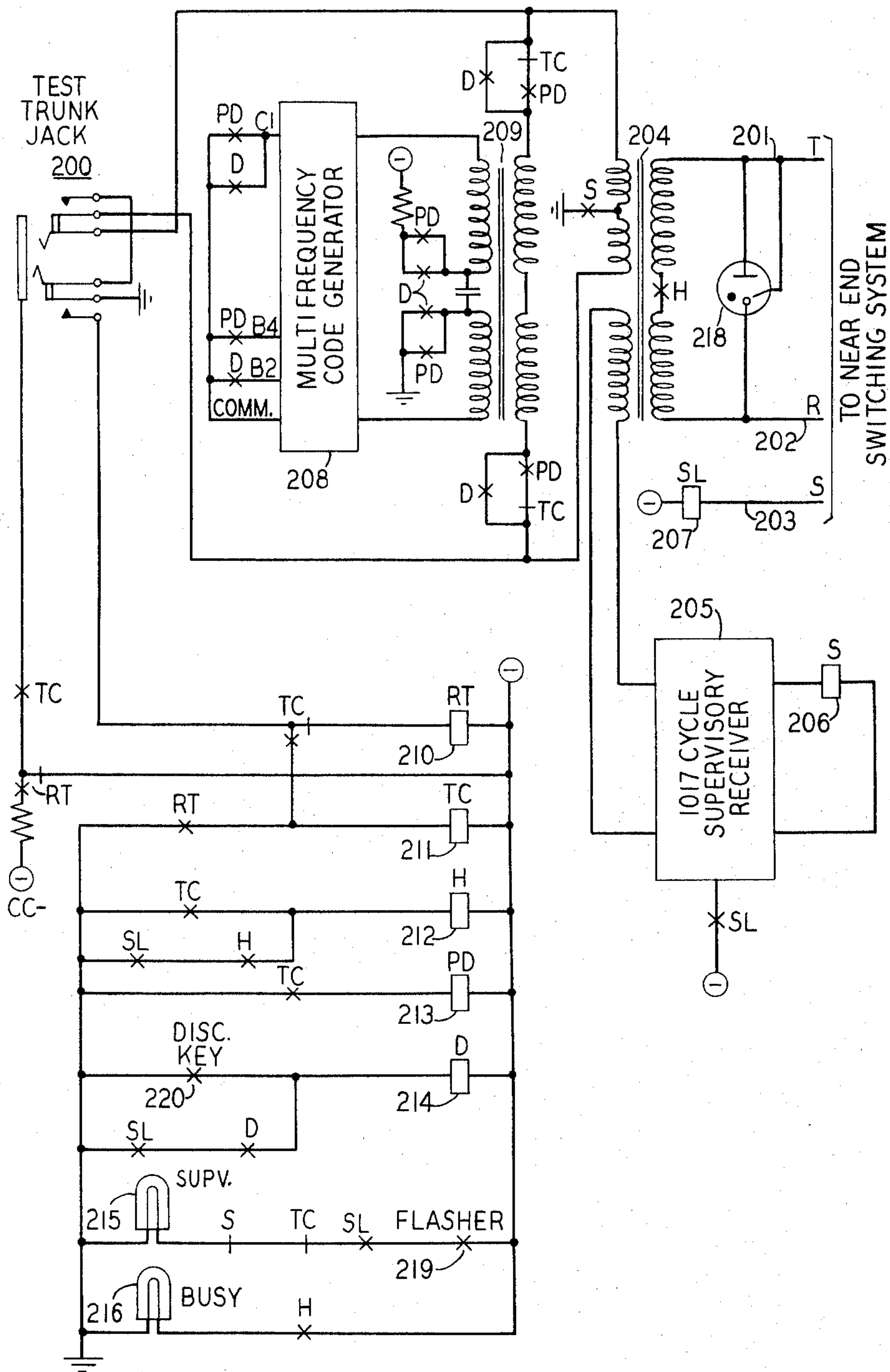
NEAR END TEST TRUNK CIRCUIT
