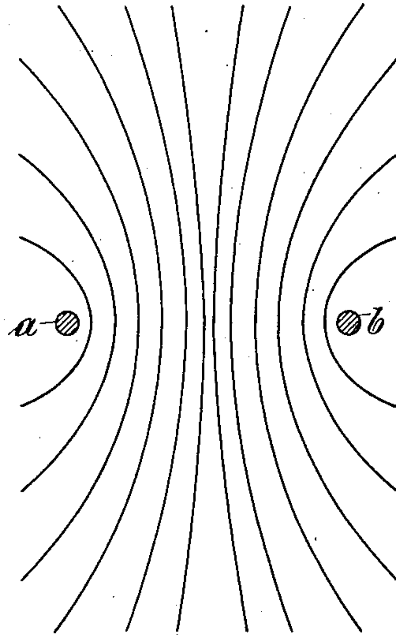
Fig. 2, Magnetic Field
