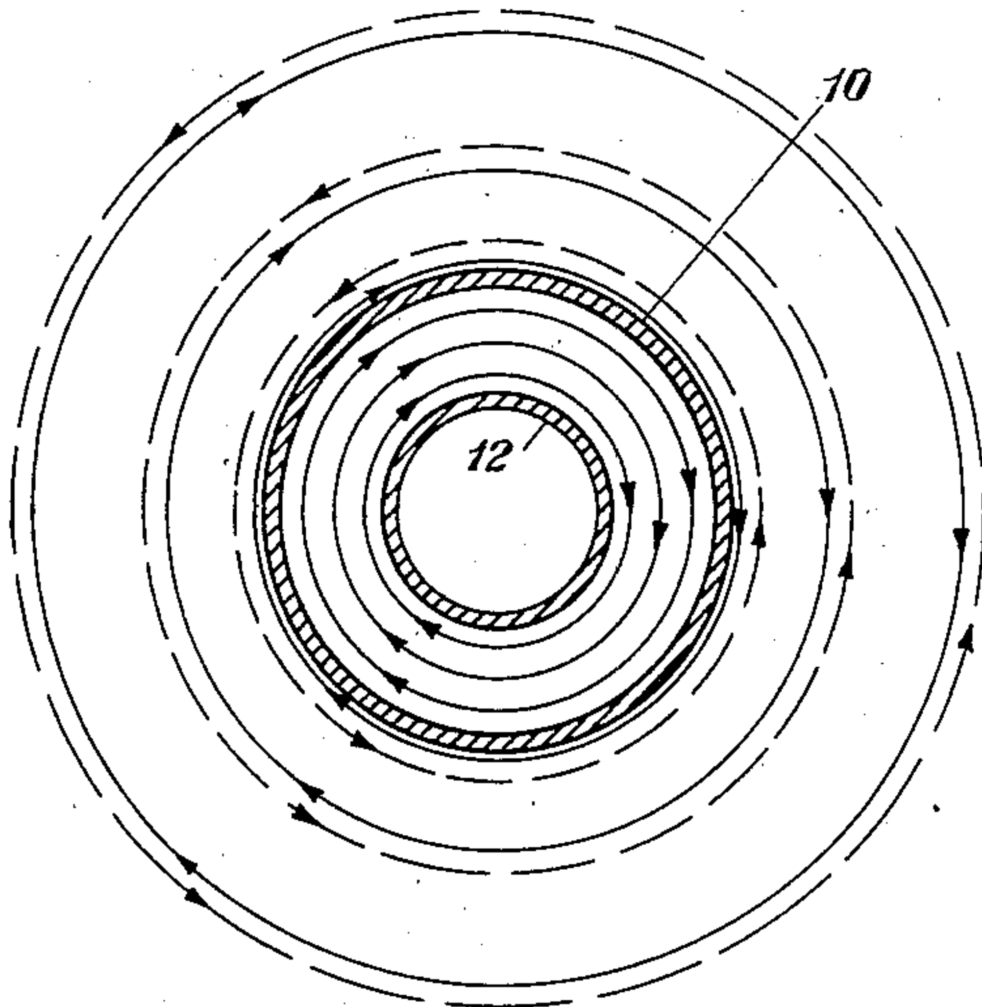
Fig. 1, Magnetic Field
