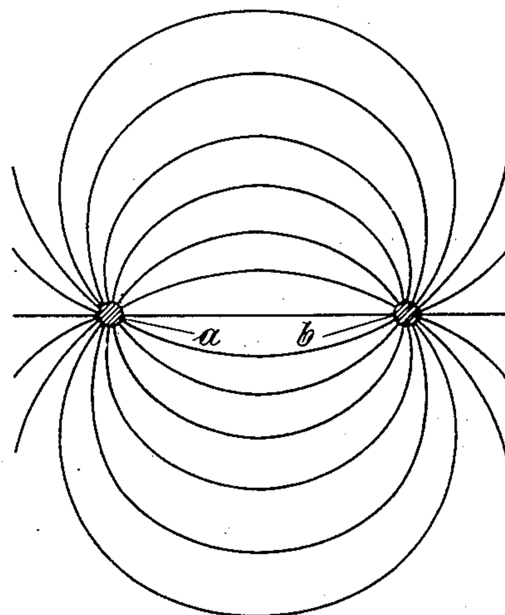
Fig. 4, Electric Field
